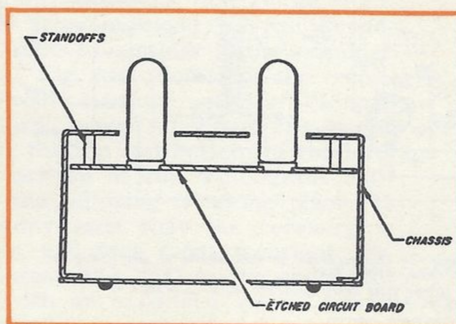
Fig. 13. Cross-section drawing of amplifier.
