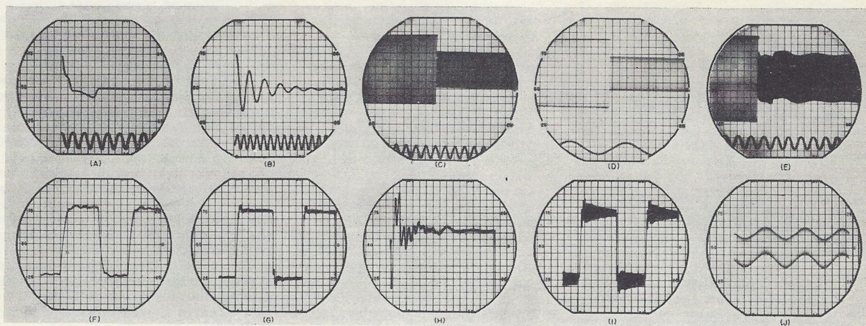
Fig. 11. (A) Step function response of the Model MLF and (B) a Williamson amplifier. (C) Overload recovery of the Model MLF and (D) with expanded time scale. (E) Overload recovery of a Williamson-type unit. (F) 10 kc. square-wave response and rise time of Model MLF and (G) Williamson-type. (H) Expanded scale square-wave top Williamson-type amplifier. (I) Square-wave ringing with capacitive load Williamson-type. (J) A Williamson-type amplifier in high-frequency oscillation.
