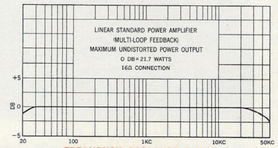
FREQUENCY RESPONSE CURVE
