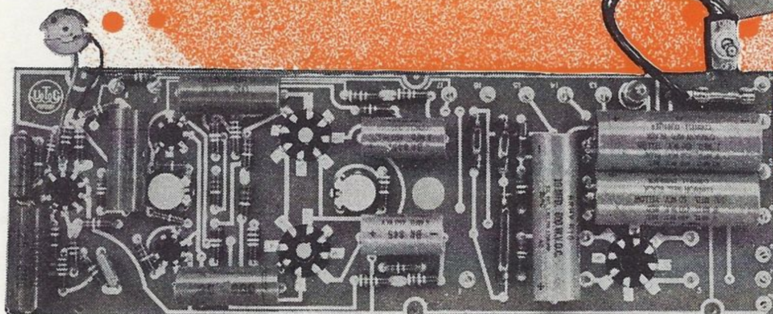
Fig. 1. Top and under chassis views of the UTC "Linear Standard" amplifier kit. Printed circuits are used for easy assembly.
