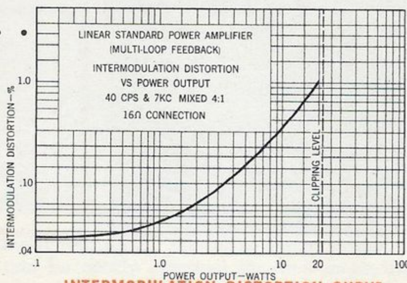
INTERMODULATION DISTORTION CURVE
