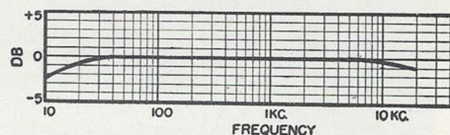
Fig. 5. Frequency response of the Model MLF at \frac{1}{2} watt output, 16 ohm connection.
