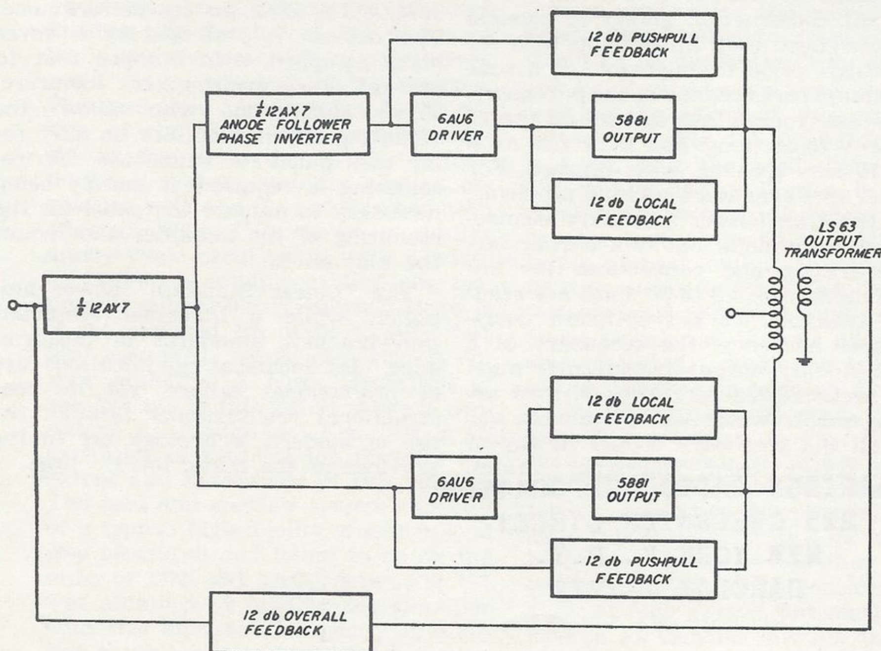
Fig. 3. Block diagram of amplifier. Other output tubes may be used. See Fig. 2.
