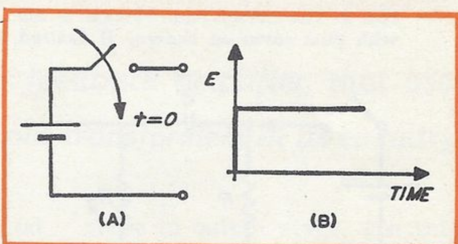
Fig. 7. Step function production and graph.
