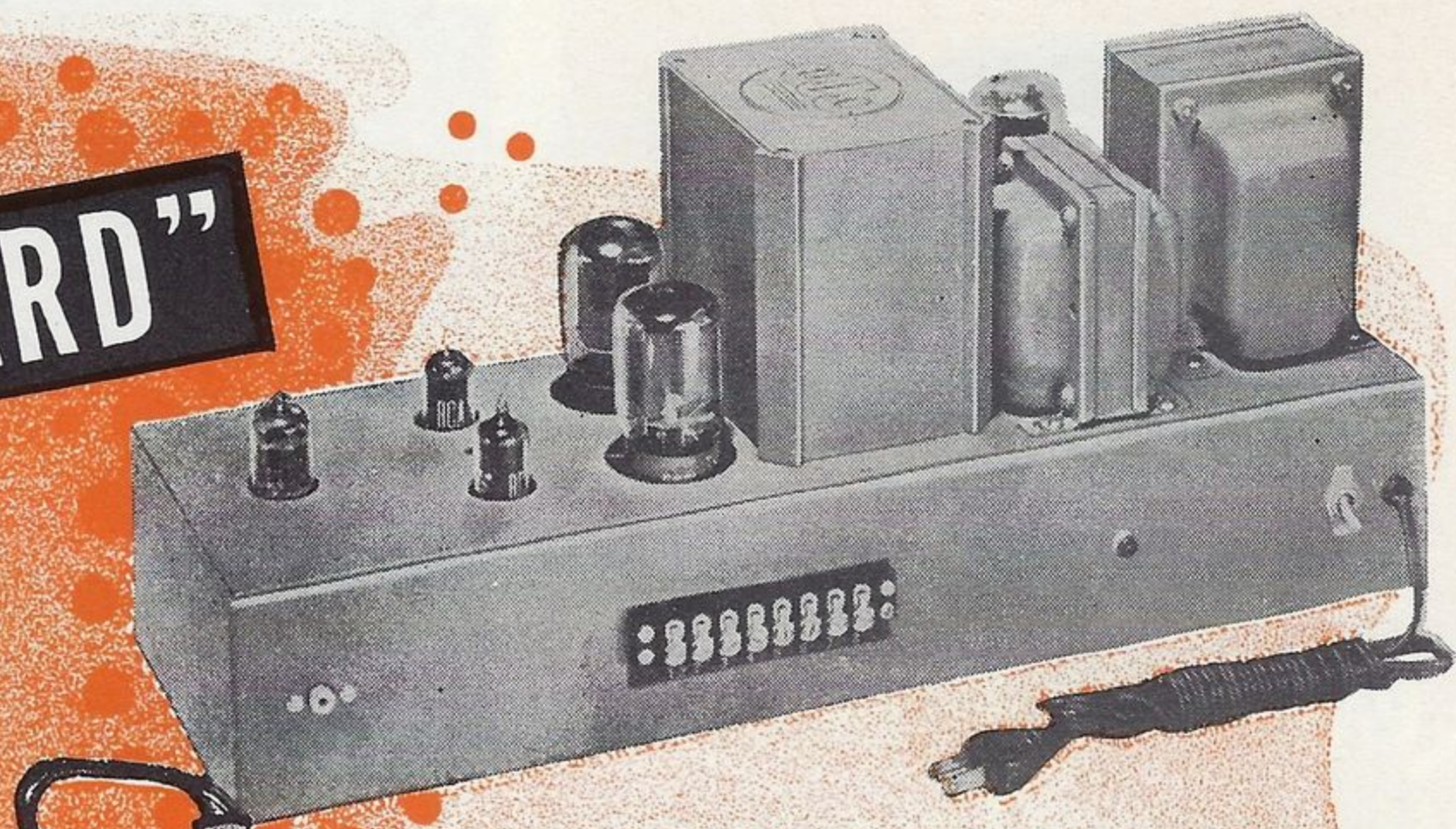
Fig. 1. Top and under chassis views of the UTC "Linear Standard" amplifier kit. Printed circuits are used for easy assembly.
