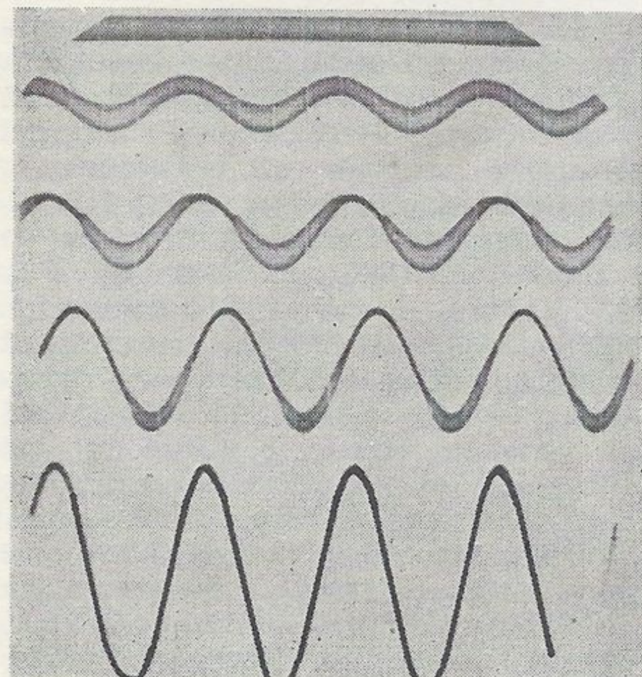
Fig. 12. Multiple oscillogram of Williamson-type amplifier output with capacitive loading as input audio signal is varied, showing the conditional stability obtained. See text for the complete discussion.
